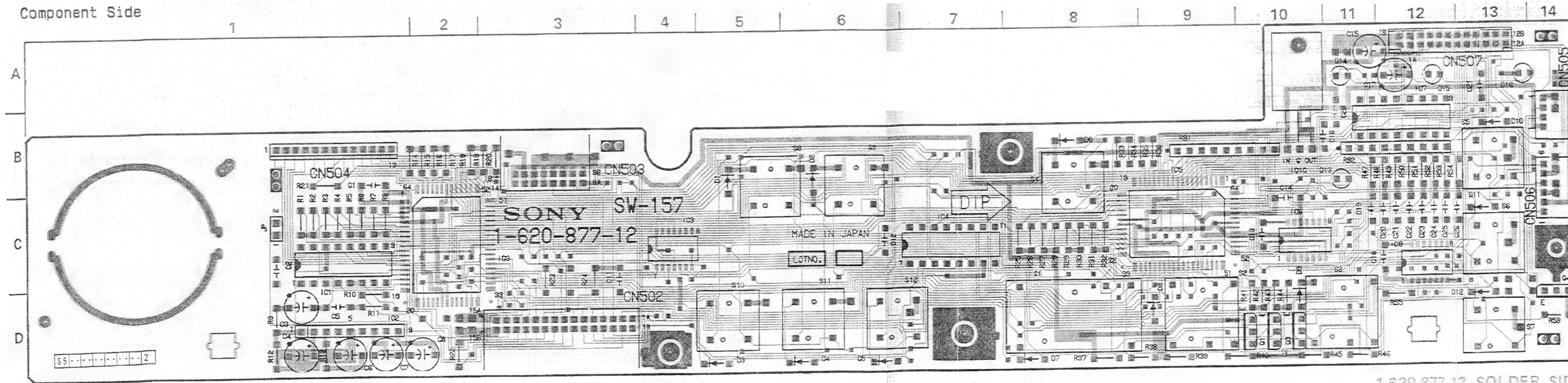
1-620-877-12 COMPONENT SIDE
